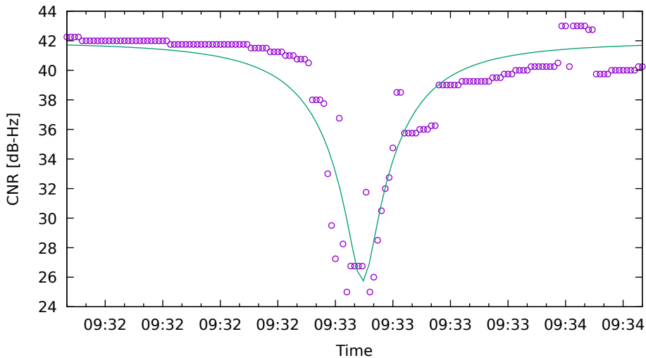
CNR fit for G03 on Xiaomi11T - drive 9 (DOY262)
