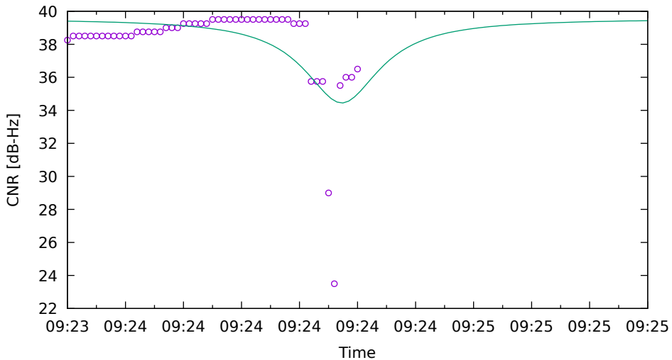
CNR fit for G04 on Xiaomi11T - drive 5 (DOY262)
