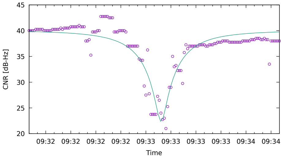
CNR fit for G04 on Xiaomi11T - drive 9 (DOY262)
