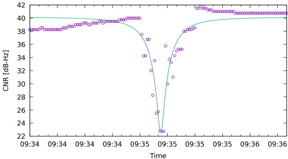
CNR fit for G17 on Xiaomi11T - drive 10 (DOY262)
