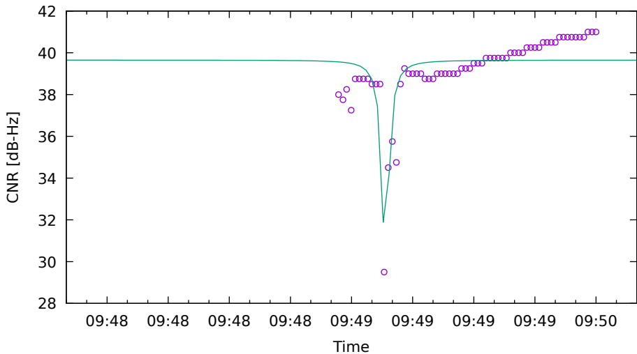
CNR fit for G17 on Xiaomi11T - drive 17 (DOY262)
