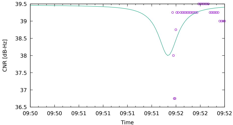
CNR fit for G17 on Xiaomi11T - drive 18 (DOY262)
