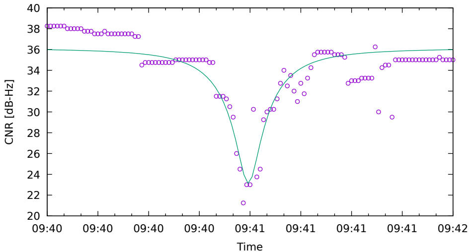
CNR fit for G19 on Xiaomi11T - drive 13 (DOY262)
