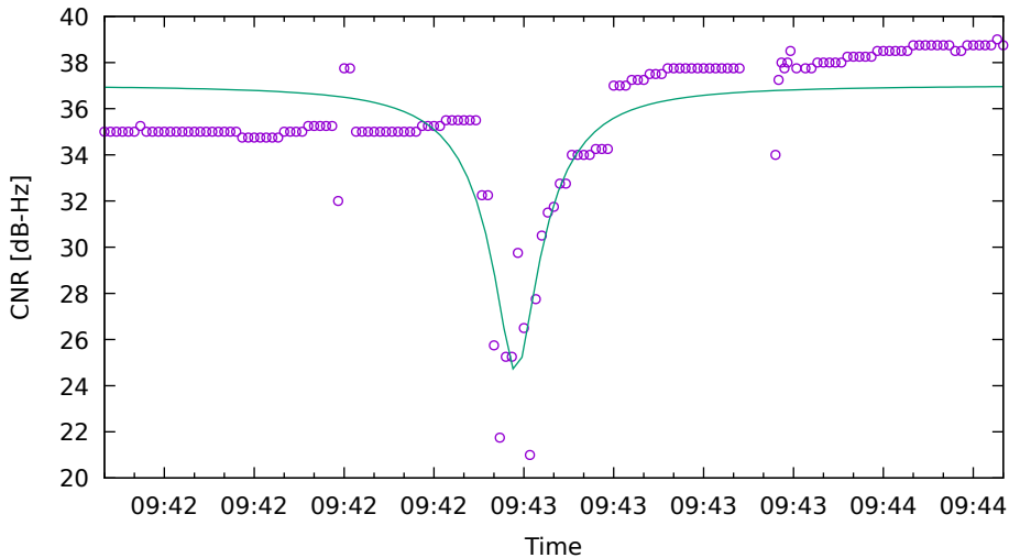
CNR fit for G19 on Xiaomi11T - drive 14 (DOY262)
