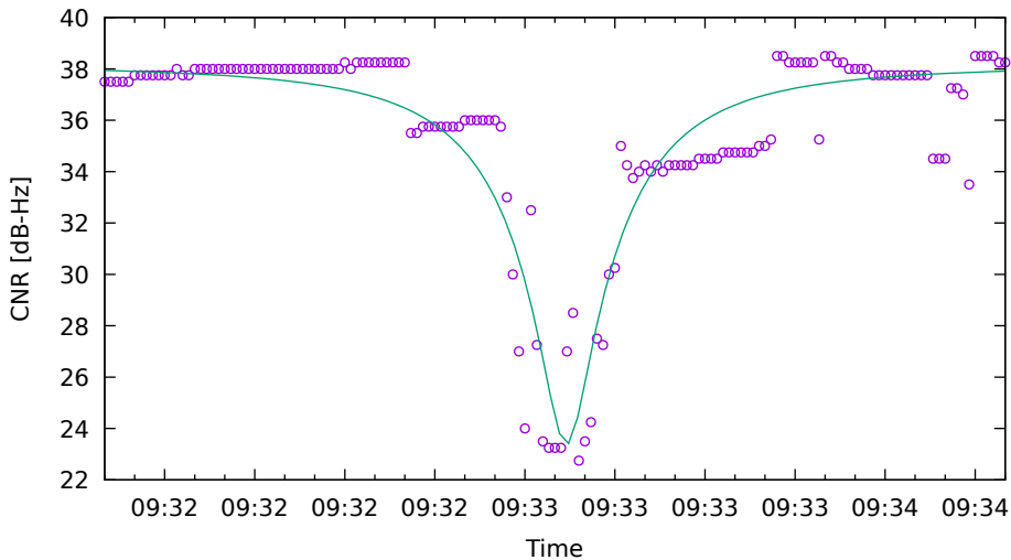
CNR fit for G19 on Xiaomi11T - drive 9 (DOY262)
