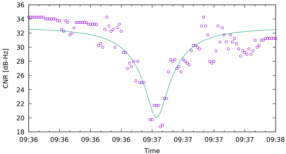
CNR fit for G21 on Xiaomi11T - drive 11 (DOY262)
