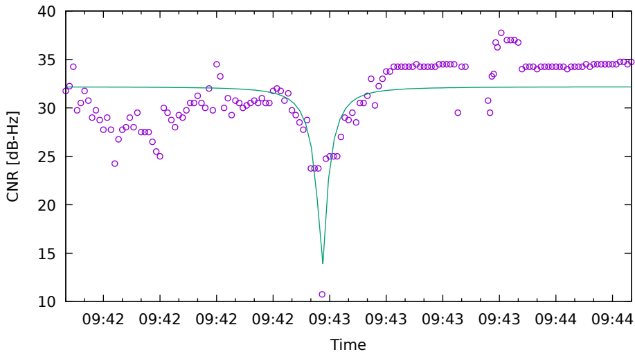
CNR fit for G21 on Xiaomi11T - drive 14 (DOY262)
