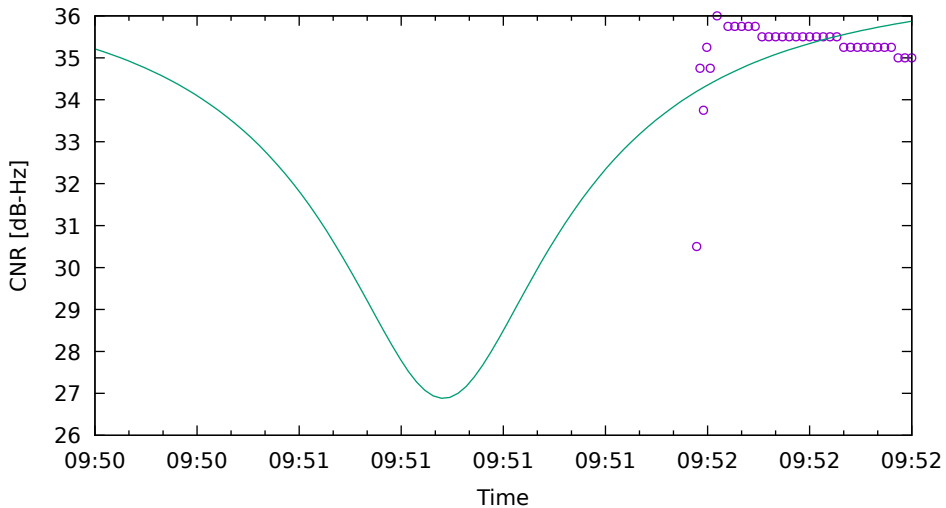
CNR fit for G21 on Xiaomi11T - drive 18 (DOY262)
