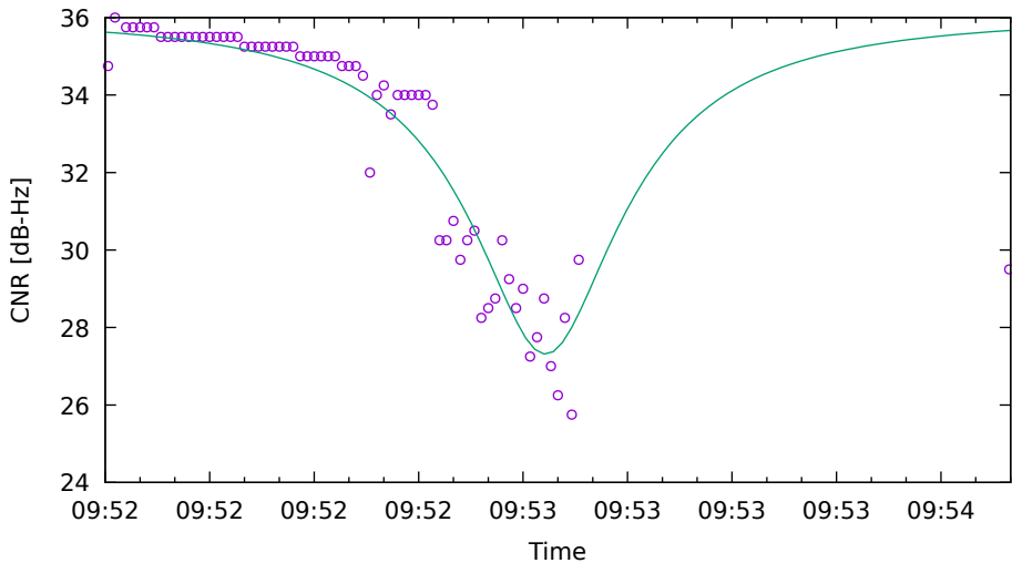
CNR fit for G21 on Xiaomi11T - drive 19 (DOY262)
