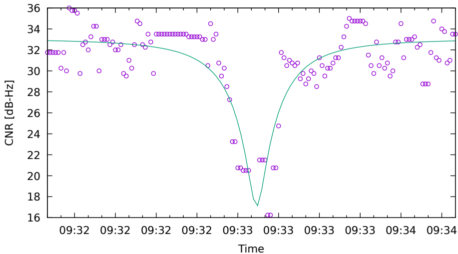
CNR fit for G21 on Xiaomi11T - drive 9 (DOY262)
