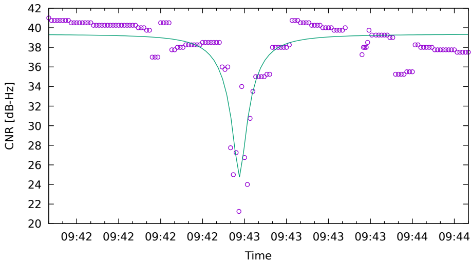
CNR fit for G22 on Xiaomi11T - drive 14 (DOY262)
