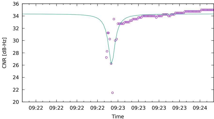
CNR fit for G31 on Xiaomi11T - drive 4 (DOY262)
