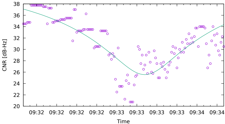
CNR fit for G31 on Xiaomi11T - drive 9 (DOY262)
