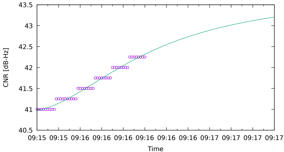
CNR fit for G32 on Xiaomi11T - drive 1 (DOY262)
