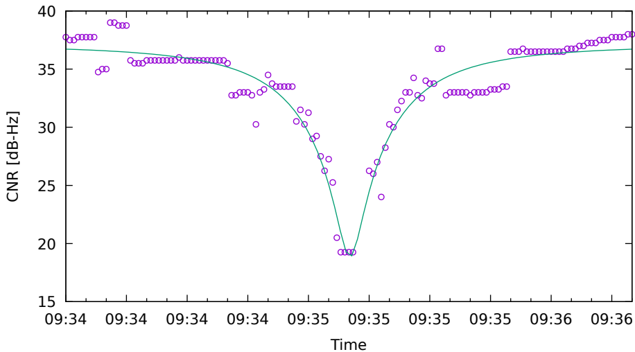
CNR fit for G32 on Xiaomi11T - drive 10 (DOY262)
