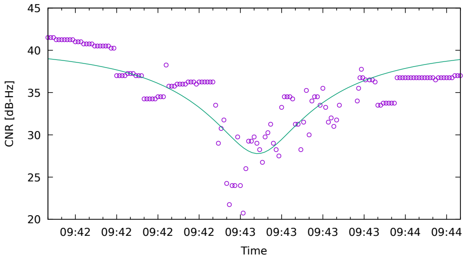
CNR fit for G32 on Xiaomi11T - drive 14 (DOY262)
