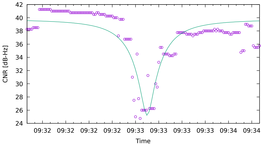
CNR fit for G32 on Xiaomi11T - drive 9 (DOY262)
