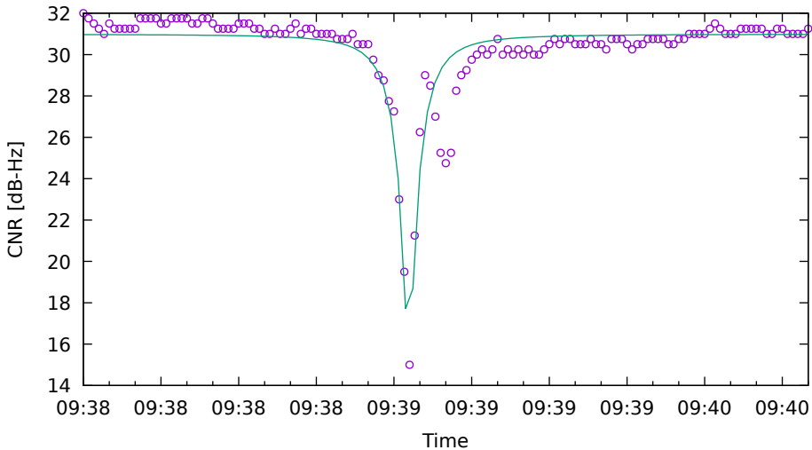
CNR fit for C09 on XiaomiMi8 - drive 12 (DOY262)
