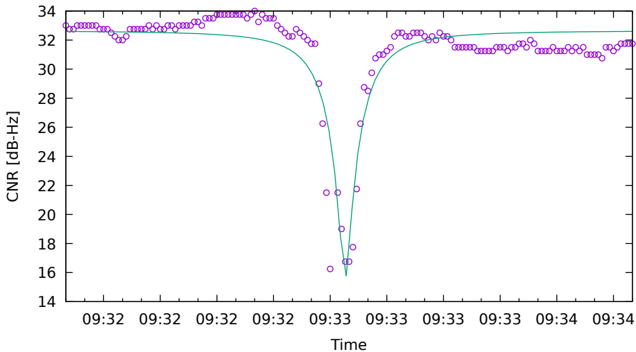
CNR fit for C09 on XiaomiMi8 - drive 9 (DOY262)
