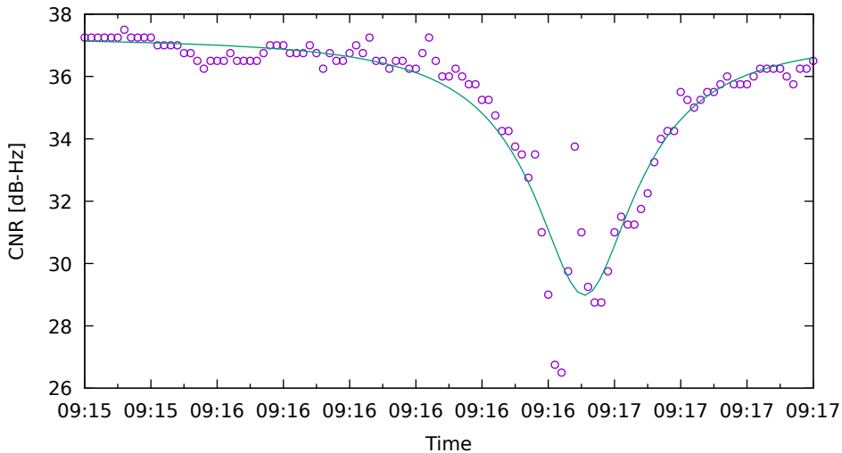
CNR fit for C11 on XiaomiMi8 - drive 1 (DOY262)
