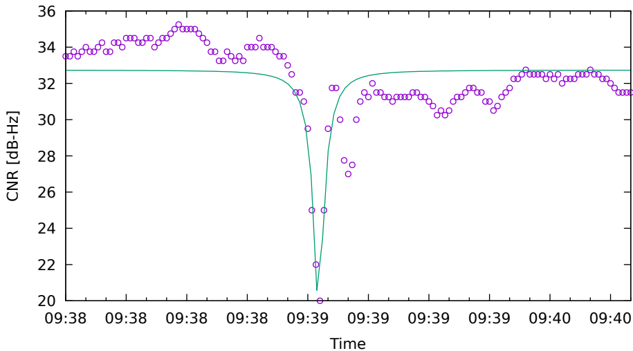
CNR fit for C11 on XiaomiMi8 - drive 12 (DOY262)
