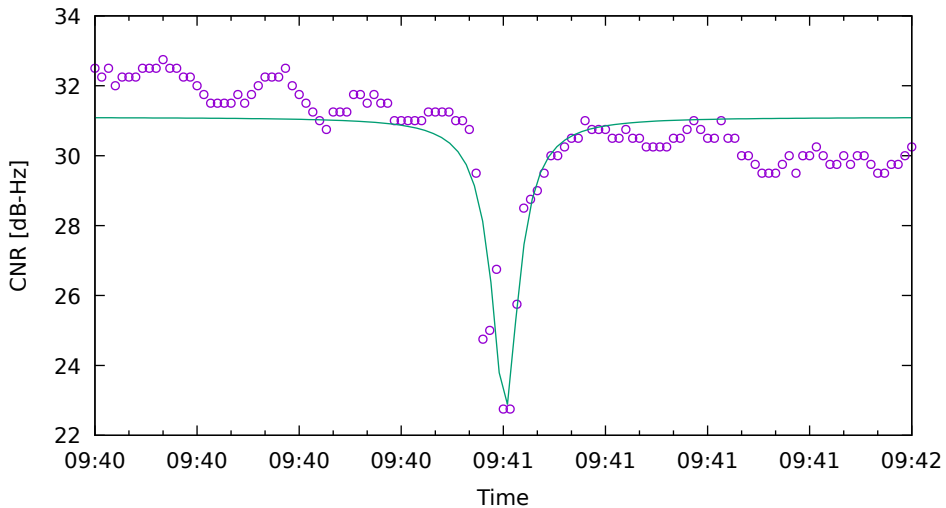
CNR fit for C11 on XiaomiMi8 - drive 13 (DOY262)
