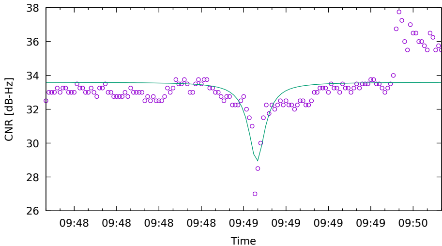
CNR fit for C11 on XiaomiMi8 - drive 17 (DOY262)
