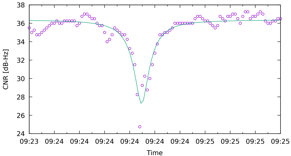
CNR fit for C11 on XiaomiMi8 - drive 5 (DOY262)
