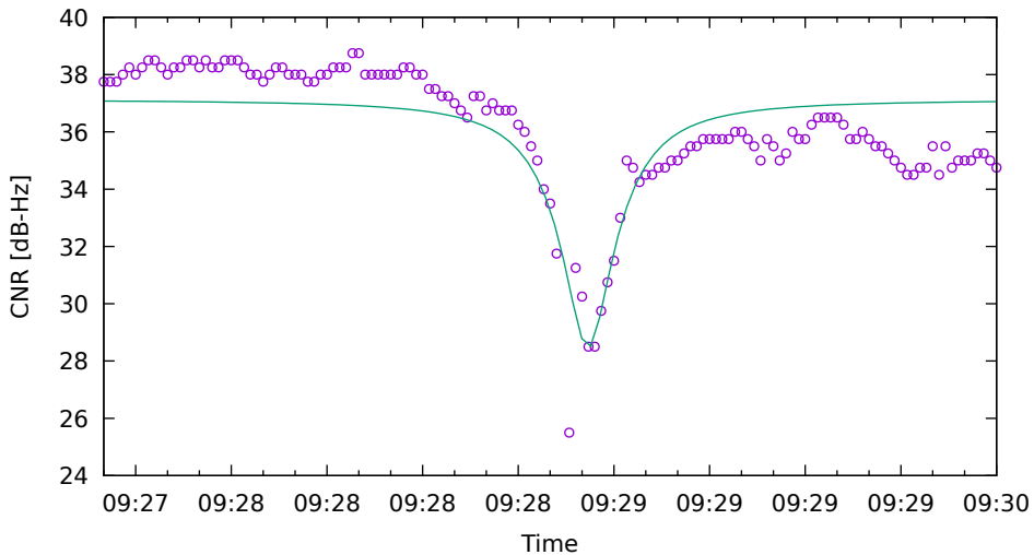
CNR fit for C11 on XiaomiMi8 - drive 7 (DOY262)
