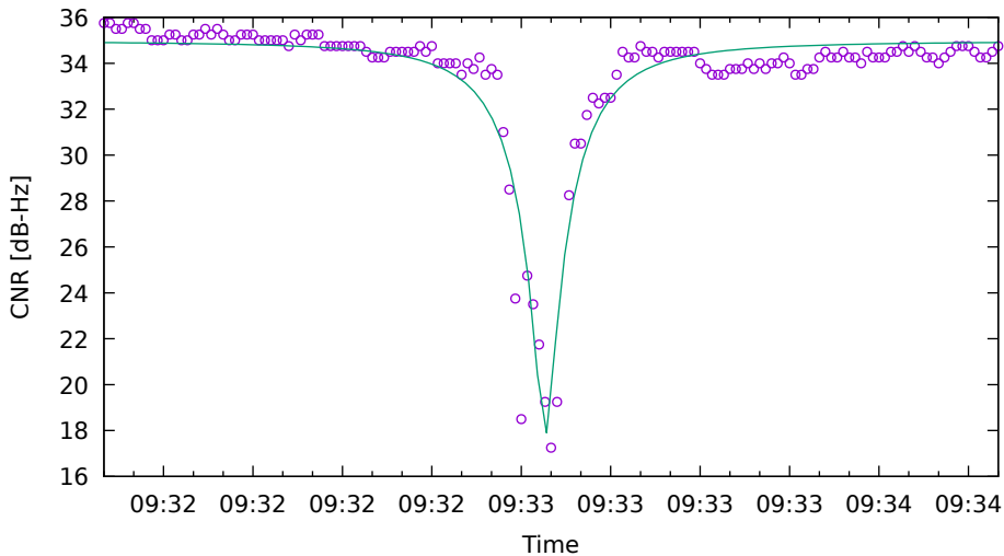
CNR fit for C11 on XiaomiMi8 - drive 9 (DOY262)
