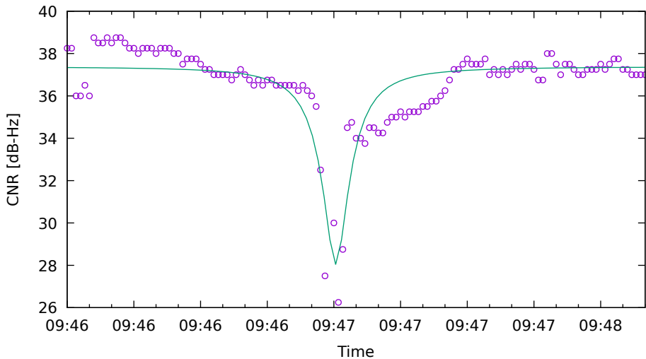
CNR fit for C27 on XiaomiMi8 - drive 16 (DOY262)
