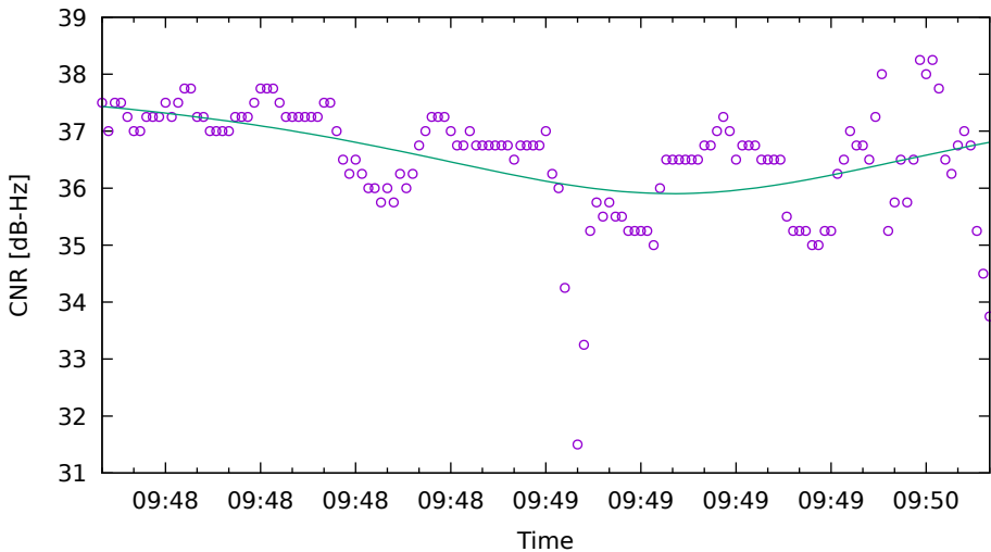
CNR fit for C27 on XiaomiMi8 - drive 17 (DOY262)
