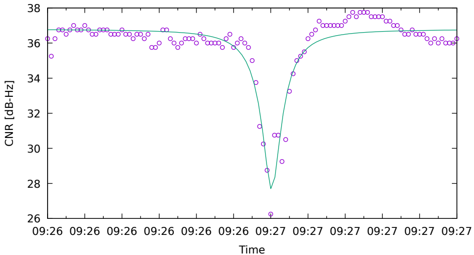
CNR fit for C27 on XiaomiMi8 - drive 6 (DOY262)
