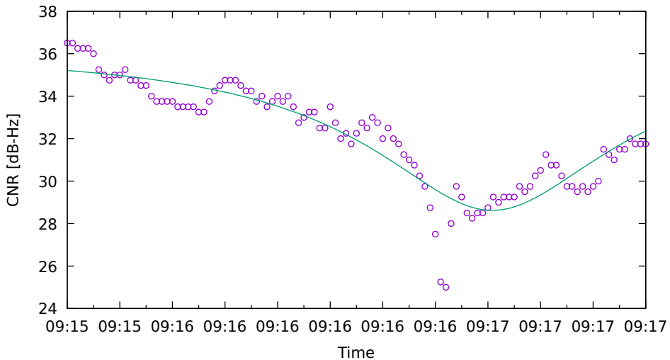
CNR fit for E04 on XiaomiMi8 - drive 1 (DOY262)
