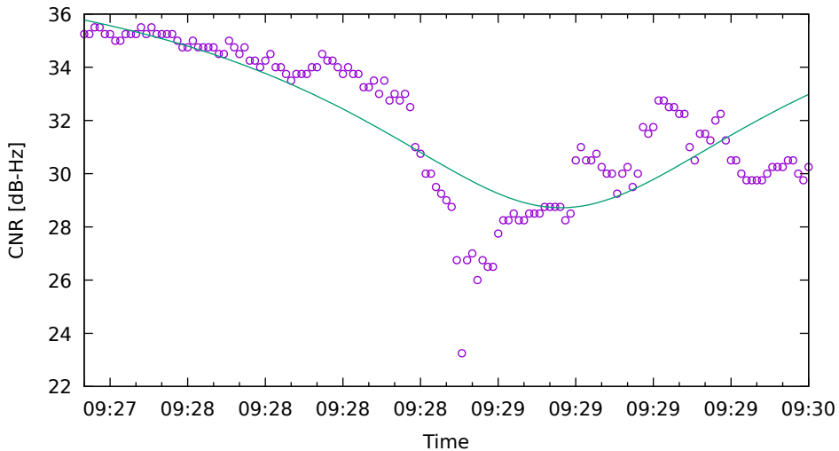
CNR fit for E04 on XiaomiMi8 - drive 7 (DOY262)
