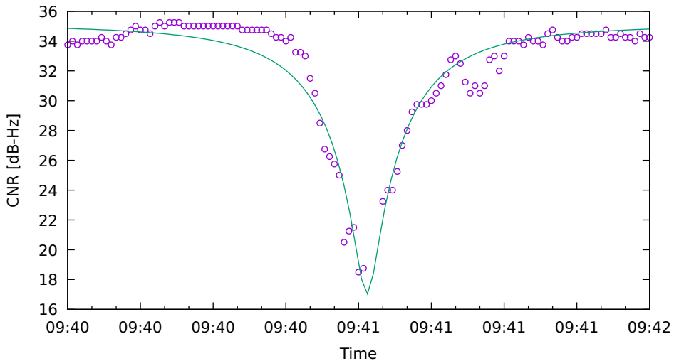
CNR fit for E05 on XiaomiMi8 - drive 13 (DOY262)
