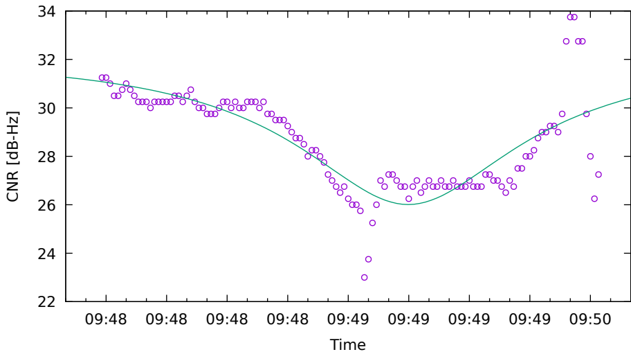
CNR fit for E05 on XiaomiMi8 - drive 17 (DOY262)
