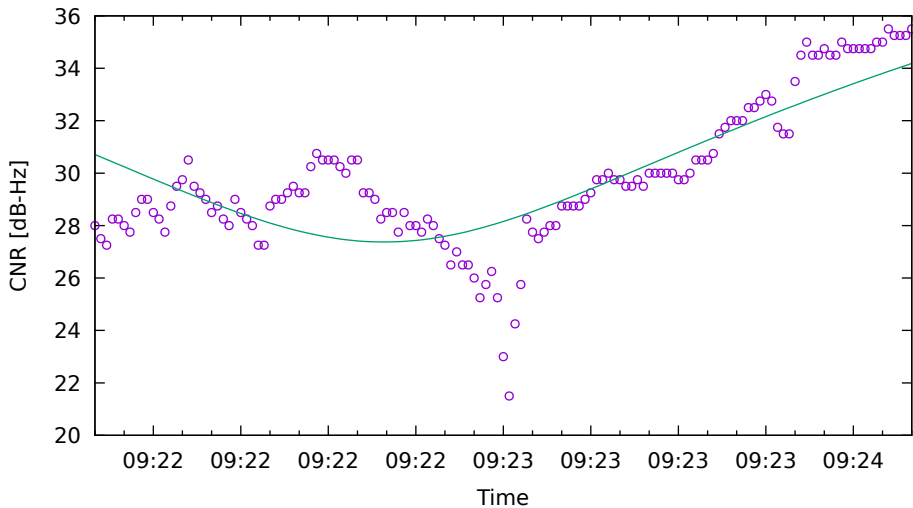
CNR fit for E05 on XiaomiMi8 - drive 4 (DOY262)
