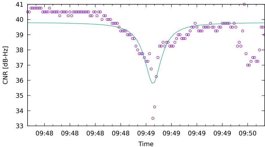
CNR fit for E09 on XiaomiMi8 - drive 17 (DOY262)
