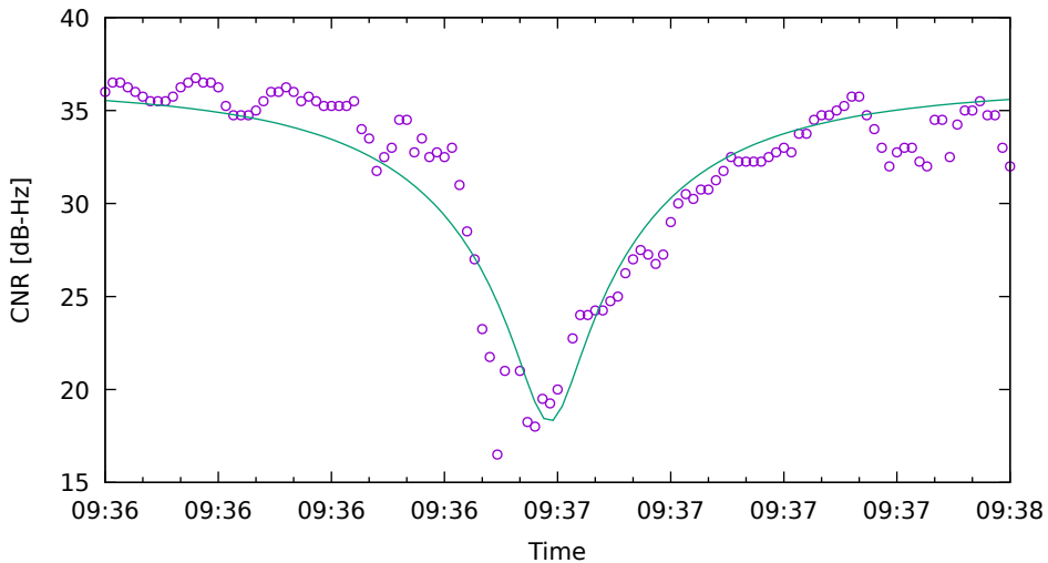
CNR fit for G01 on XiaomiMi8 - drive 11 (DOY262)
