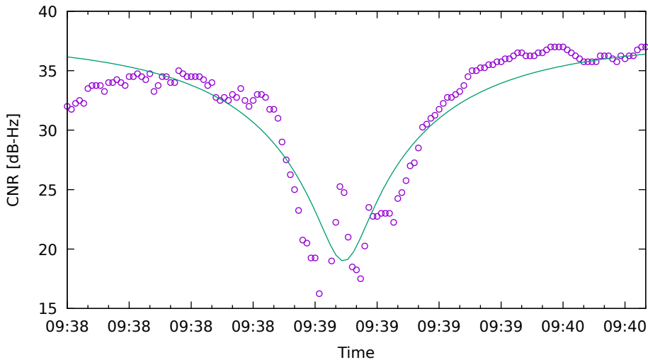
CNR fit for G01 on XiaomiMi8 - drive 12 (DOY262)
