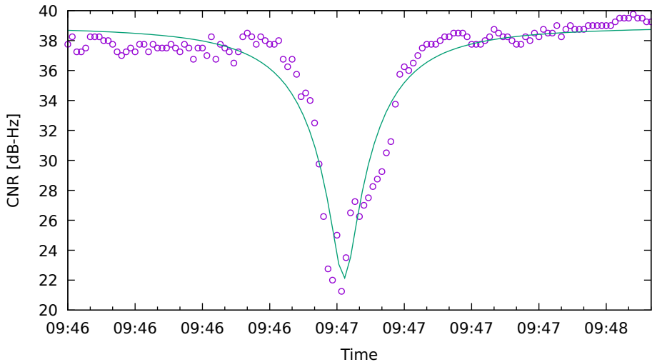
CNR fit for G01 on XiaomiMi8 - drive 16 (DOY262)
