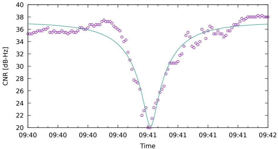
CNR fit for G03 on XiaomiMi8 - drive 13 (DOY262)
