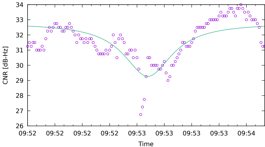
CNR fit for G03 on XiaomiMi8 - drive 19 (DOY262)
