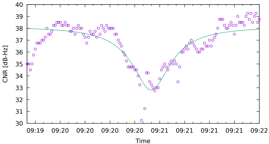
CNR fit for G03 on XiaomiMi8 - drive 3 (DOY262)
