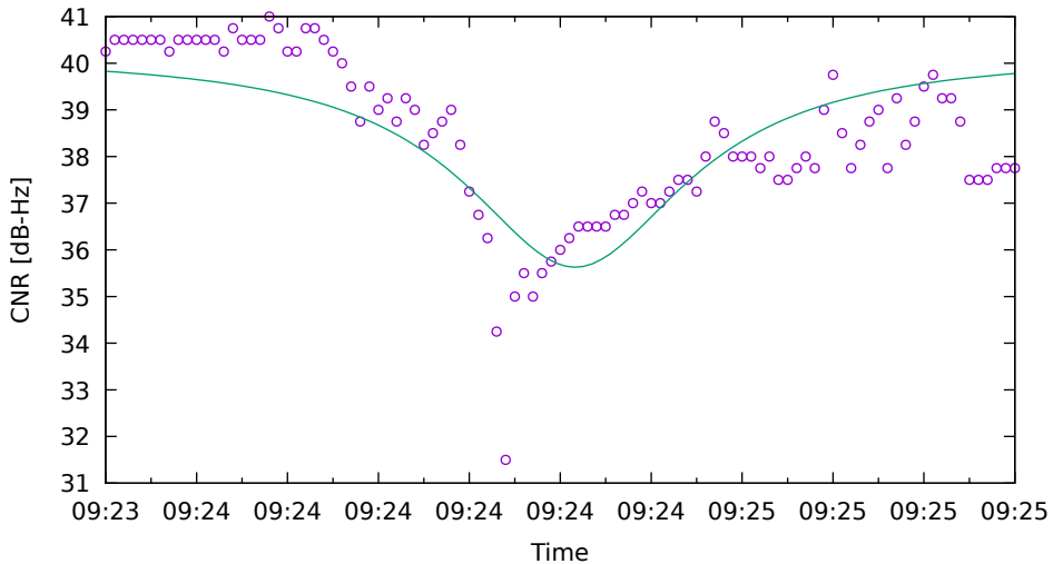
CNR fit for G03 on XiaomiMi8 - drive 5 (DOY262)
