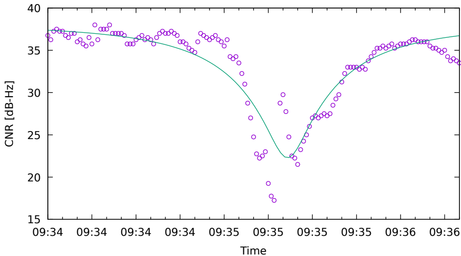
CNR fit for G08 on XiaomiMi8 - drive 10 (DOY262)
