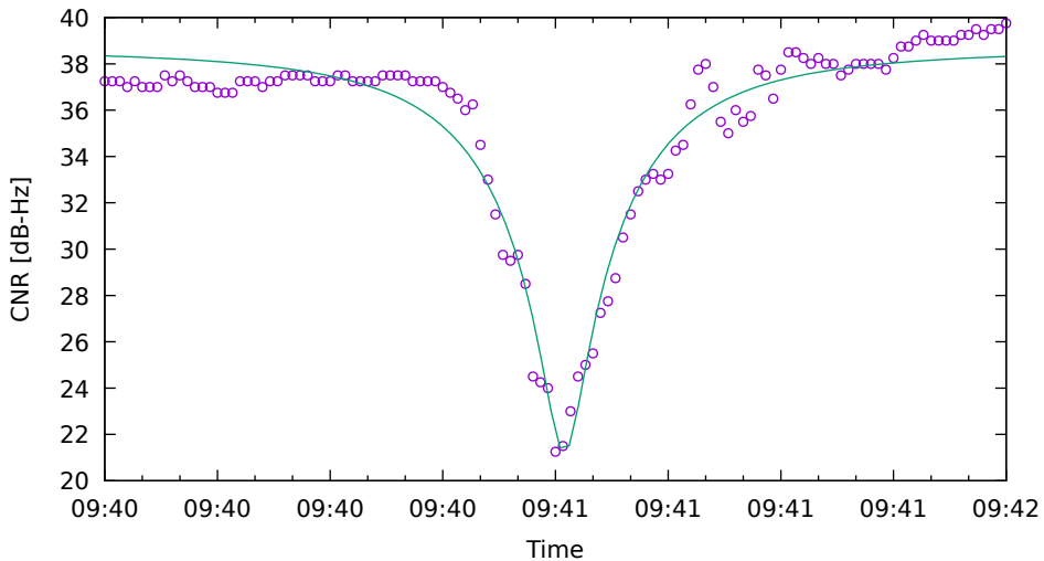
CNR fit for G08 on XiaomiMi8 - drive 13 (DOY262)
