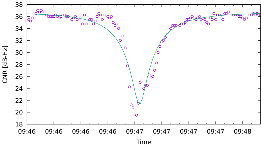
CNR fit for G08 on XiaomiMi8 - drive 16 (DOY262)
