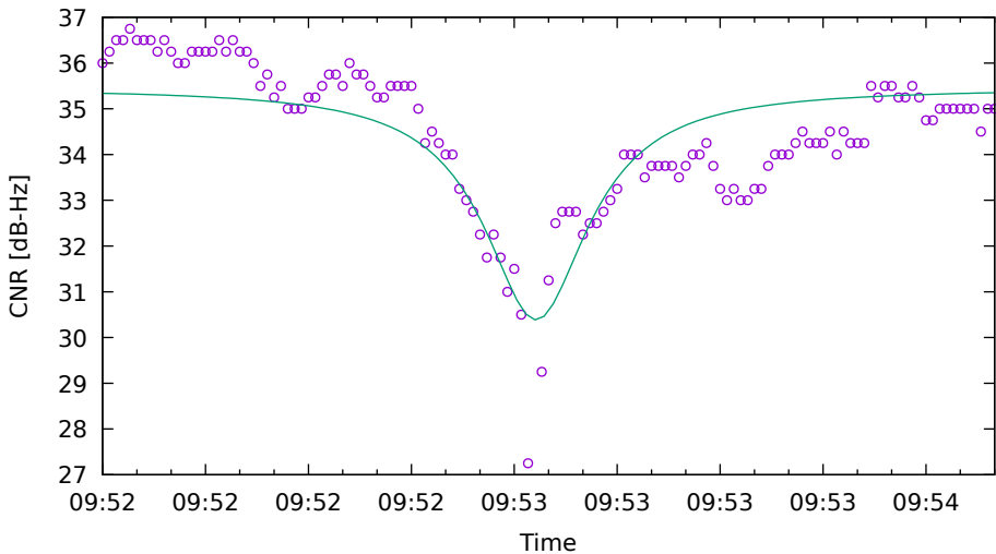
CNR fit for G08 on XiaomiMi8 - drive 19 (DOY262)
